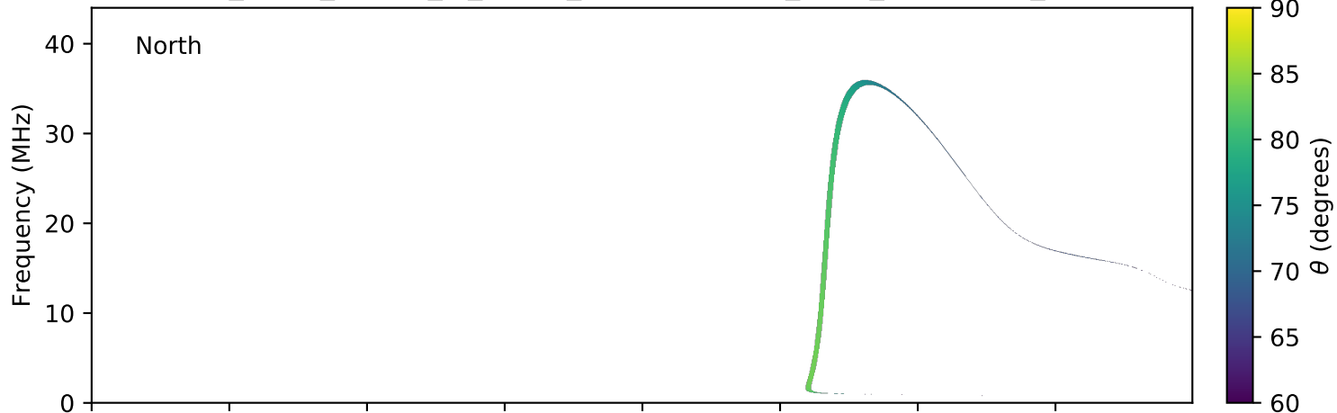
expres_earth_jupiter_io_jrm09_lossc-wid1deg_3kev_20160515_v01.cdf
