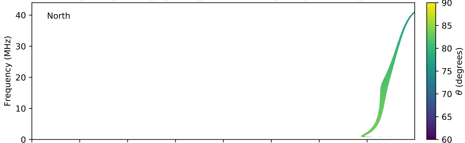
expres_earth_jupiter_io_jrm09_lossc-wid1deg_3kev_20160513_v01.cdf
