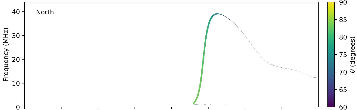
expres_earth_jupiter_io_jrm09_lossc-wid1deg_3kev_20160508_v01.cdf
