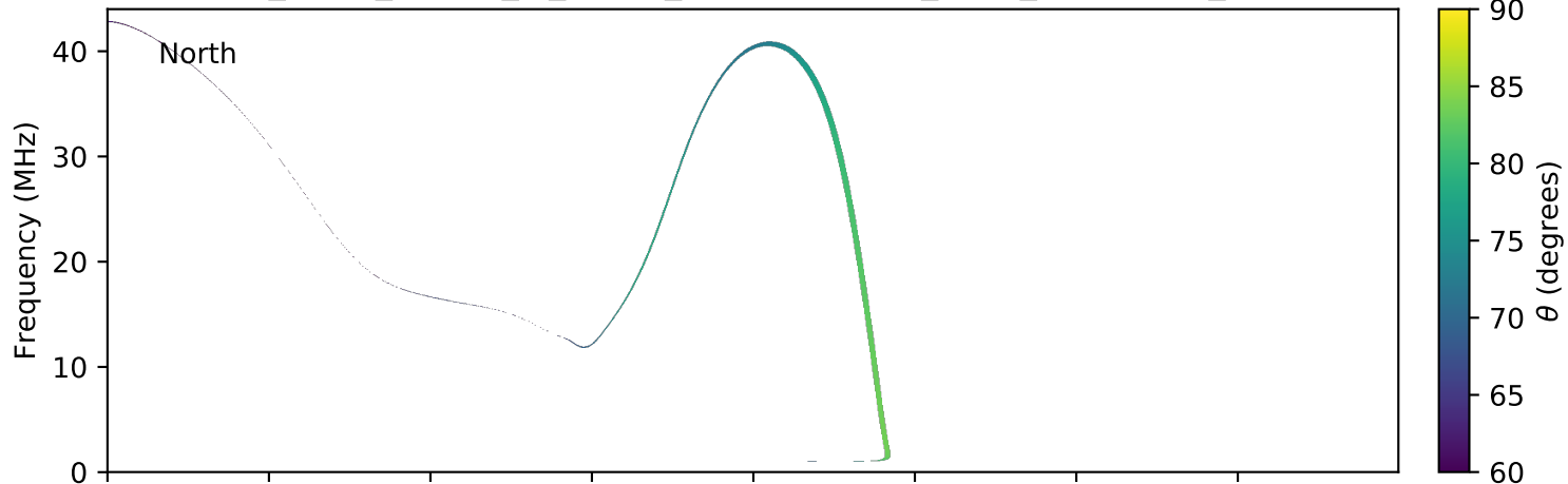
expres_earth_jupiter_io_jrm09_lossc-wid1deg_3kev_20160507_v01.cdf
