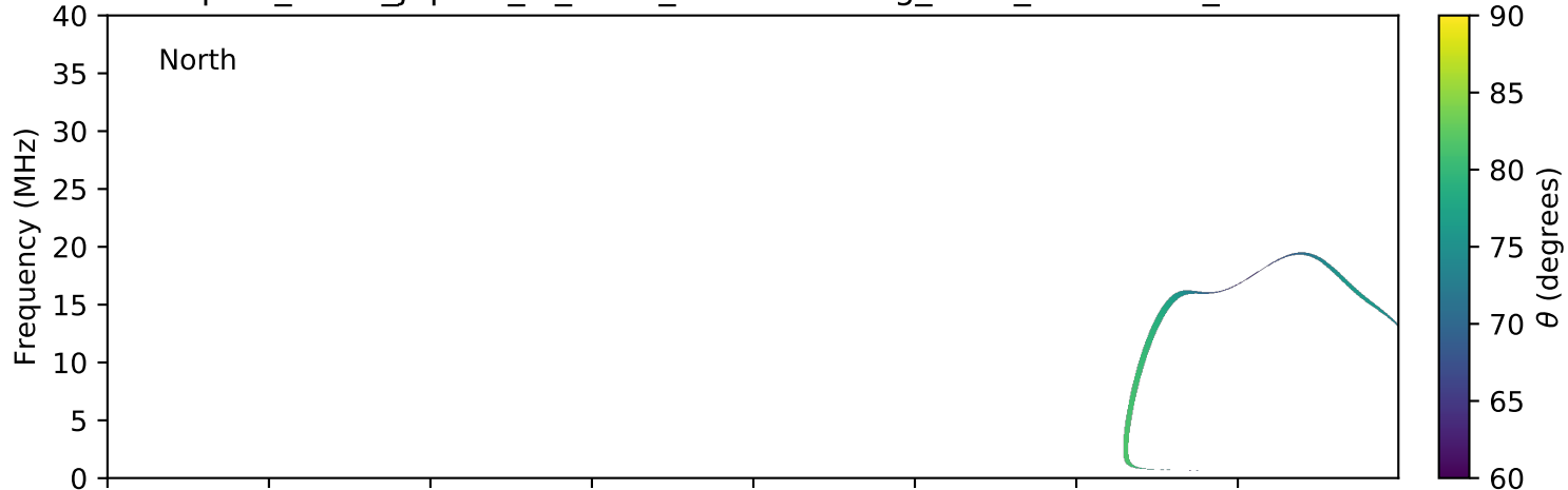
expres_earth_jupiter_io_isaac_lossc-wid1deg_5kev_20160529_v01.cdf
