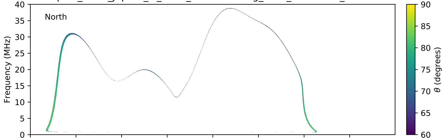
expres_earth_jupiter_io_isaac_lossc-wid1deg_5kev_20160528_v01.cdf
