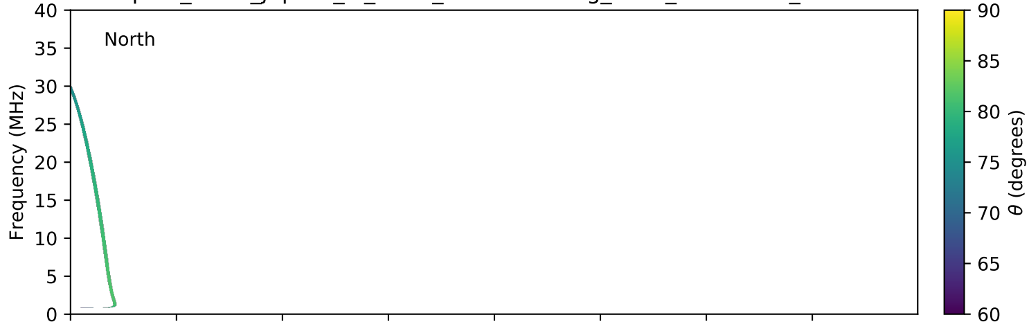
expres_earth_jupiter_io_isaac_lossc-wid1deg_5kev_20160527_v01.cdf
