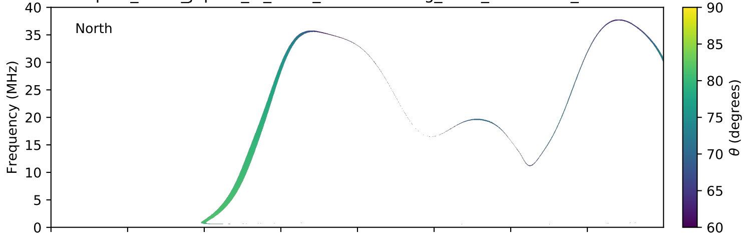
expres_earth_jupiter_io_isaac_lossc-wid1deg_5kev_20160526_v01.cdf
