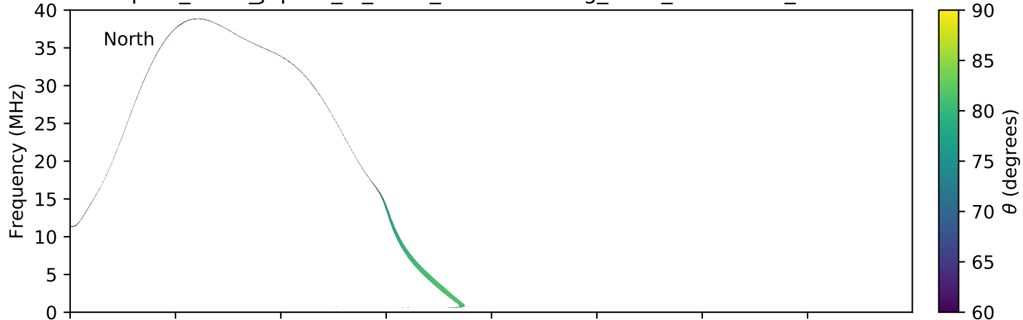
expres_earth_jupiter_io_isaac_lossc-wid1deg_5kev_20160523_v01.cdf
