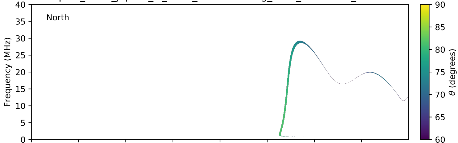
expres_earth_jupiter_io_isaac_lossc-wid1deg_5kev_20160515_v01.cdf
