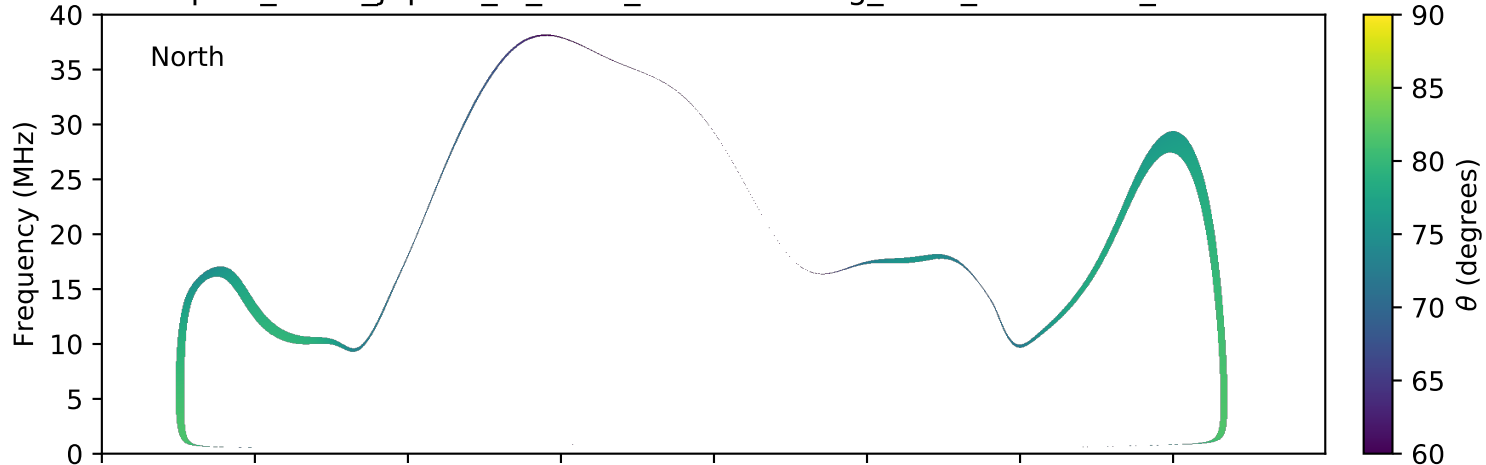
expres_earth_jupiter_io_isaac_lossc-wid1deg_5kev_20160512_v01.cdf
