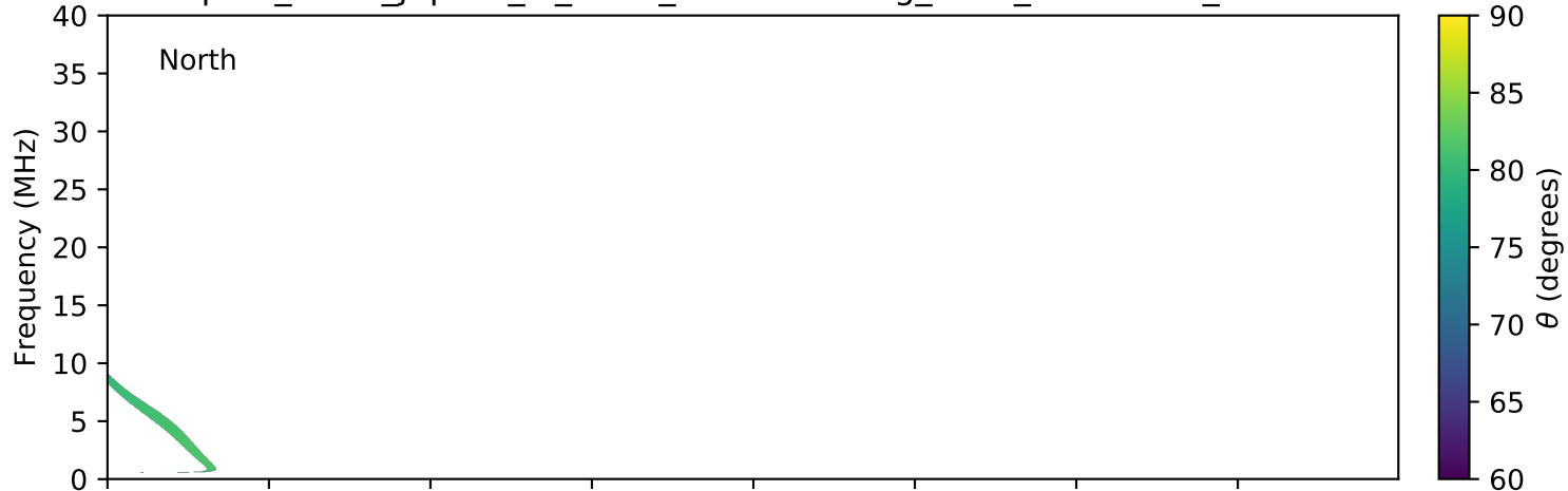
expres_earth_jupiter_io_isaac_lossc-wid1deg_5kev_20160511_v01.cdf
