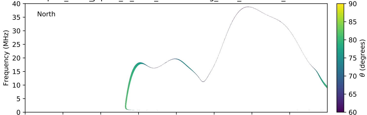
expres_earth_jupiter_io_isaac_lossc-wid1deg_5kev_20160510_v01.cdf
