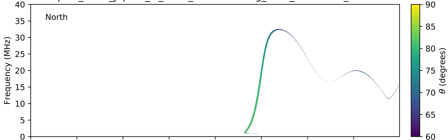
expres_earth_jupiter_io_isaac_lossc-wid1deg_5kev_20160508_v01.cdf
