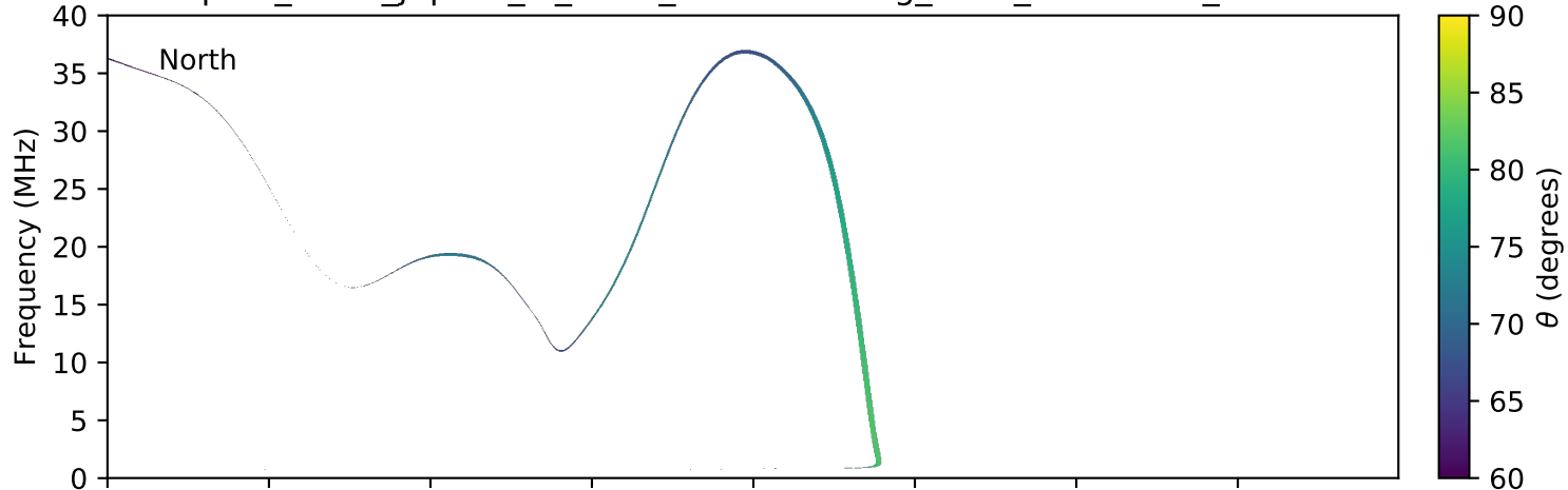
expres_earth_jupiter_io_isaac_lossc-wid1deg_5kev_20160507_v01.cdf
