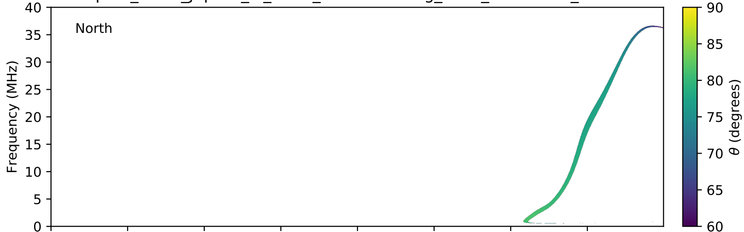
expres_earth_jupiter_io_isaac_lossc-wid1deg_5kev_20160506_v01.cdf
