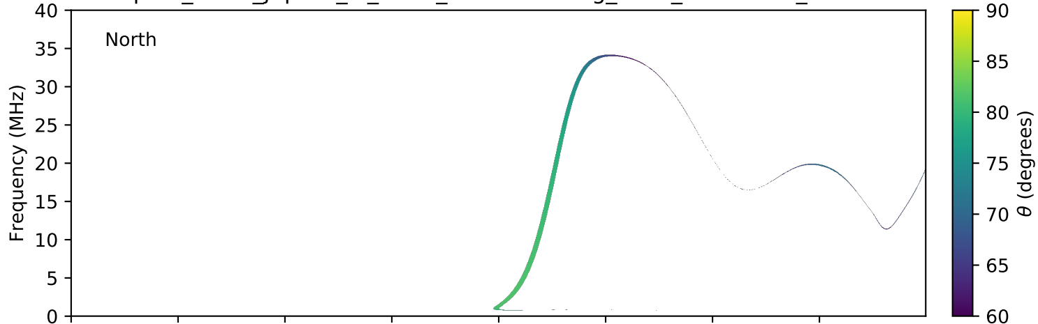
expres_earth_jupiter_io_isaac_lossc-wid1deg_5kev_20160501_v01.cdf
