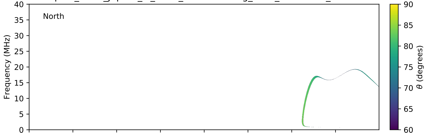
expres_earth_jupiter_io_isaac_lossc-wid1deg_3kev_20160529_v01.cdf
