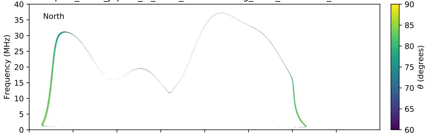
expres_earth_jupiter_io_isaac_lossc-wid1deg_3kev_20160528_v01.cdf
