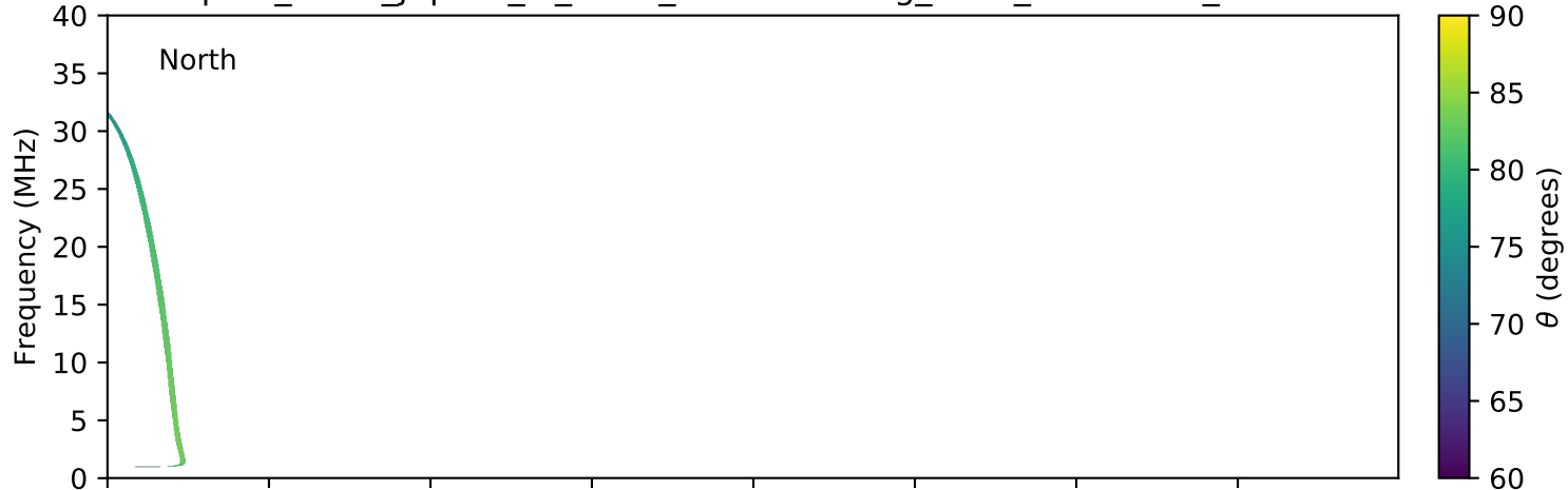
expres_earth_jupiter_io_isaac_lossc-wid1deg_3kev_20160527_v01.cdf
