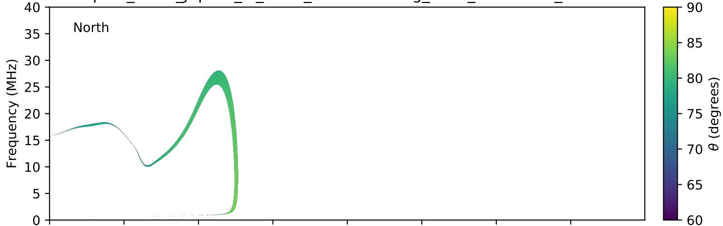
expres_earth_jupiter_io_isaac_lossc-wid1deg_3kev_20160525_v01.cdf
