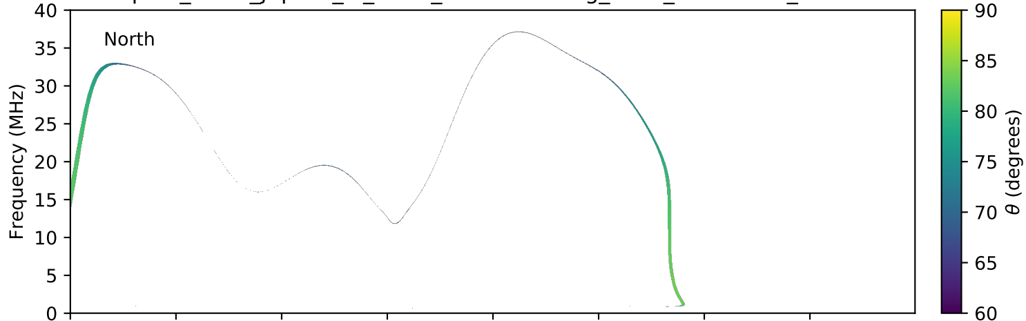
expres_earth_jupiter_io_isaac_lossc-wid1deg_3kev_20160521_v01.cdf
