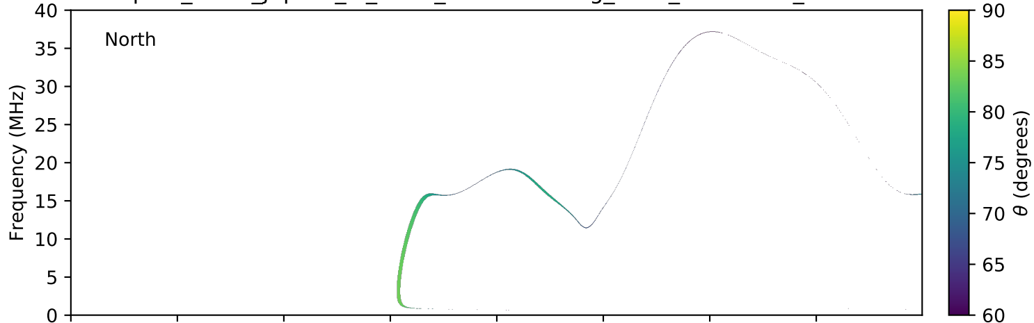
expres_earth_jupiter_io_isaac_lossc-wid1deg_3kev_20160517_v01.cdf
