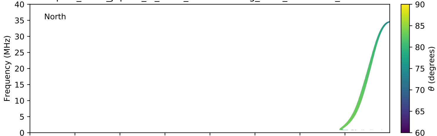
expres_earth_jupiter_io_isaac_lossc-wid1deg_3kev_20160513_v01.cdf
