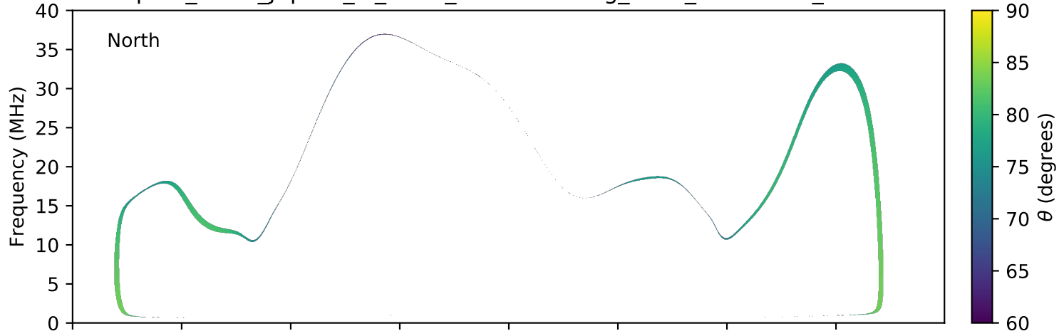
expres_earth_jupiter_io_isaac_lossc-wid1deg_3kev_20160512_v01.cdf
