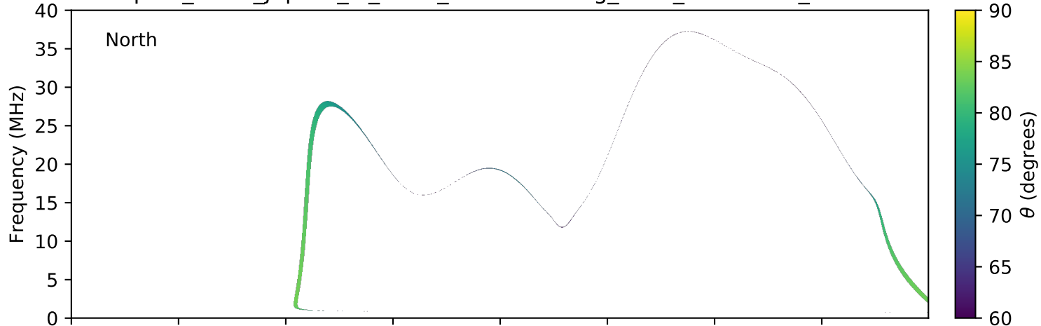
expres_earth_jupiter_io_isaac_lossc-wid1deg_3kev_20160503_v01.cdf
