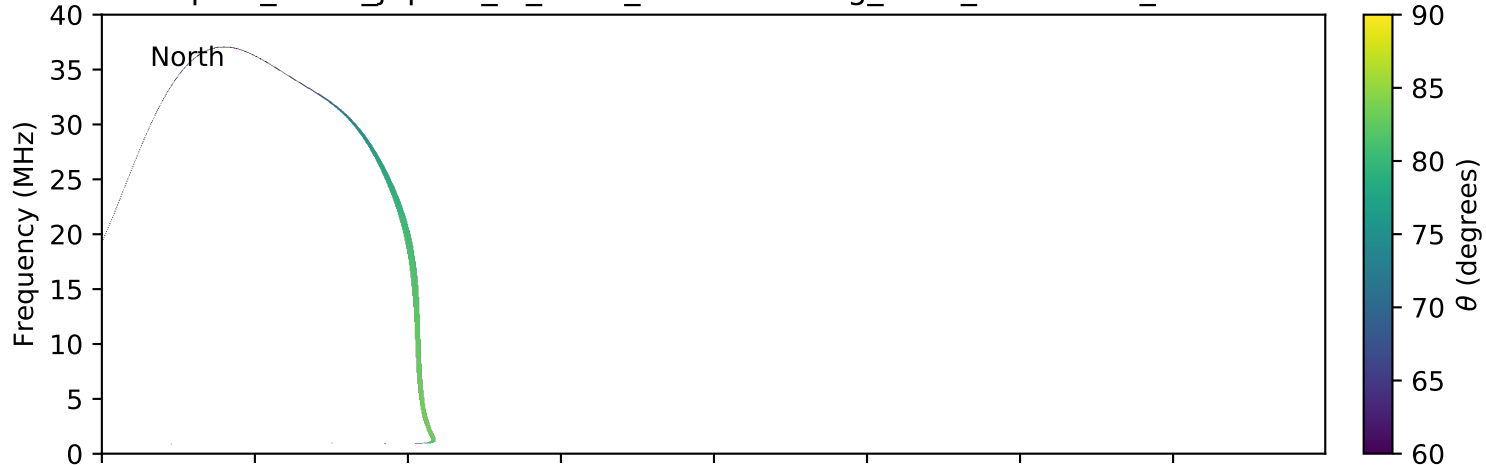
expres_earth_jupiter_io_isaac_lossc-wid1deg_3kev_20160502_v01.cdf
