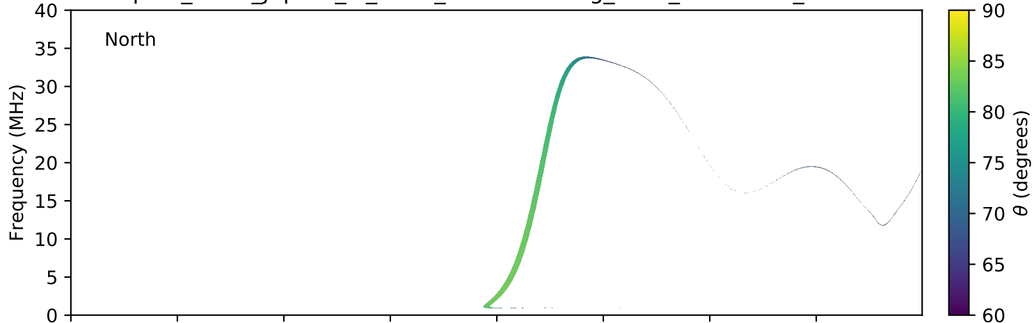
expres_earth_jupiter_io_isaac_lossc-wid1deg_3kev_20160501_v01.cdf
