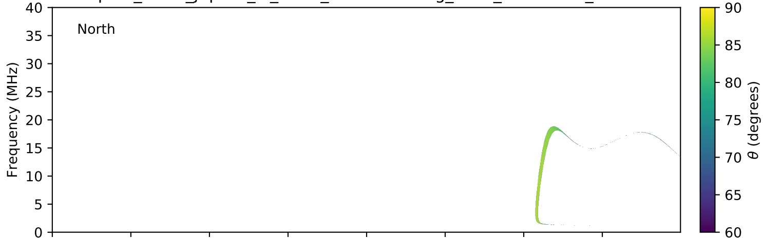
expres_earth_jupiter_io_isaac_lossc-wid1deg_1kev_20160529_v01.cdf
