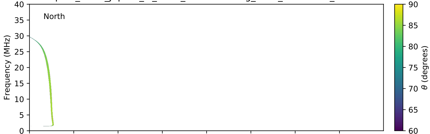
expres_earth_jupiter_io_isaac_lossc-wid1deg_1kev_20160527_v01.cdf
