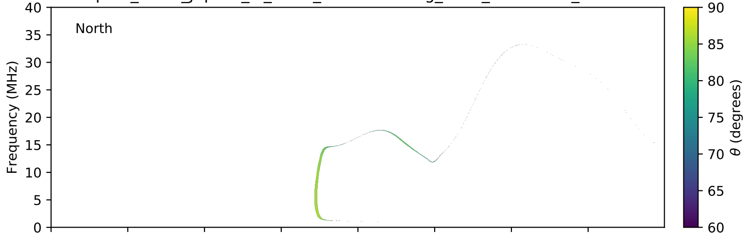
expres_earth_jupiter_io_isaac_lossc-wid1deg_1kev_20160524_v01.cdf
