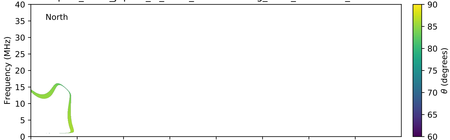
expres_earth_jupiter_io_isaac_lossc-wid1deg_1kev_20160511_v01.cdf
