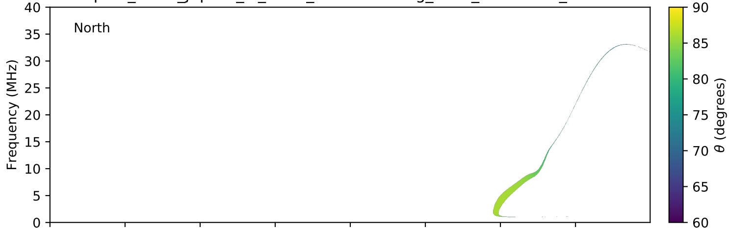
expres_earth_jupiter_io_isaac_lossc-wid1deg_1kev_20160506_v01.cdf
