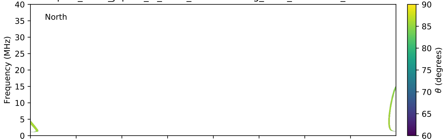
expres_earth_jupiter_io_isaac_lossc-wid1deg_1kev_20160504_v01.cdf
