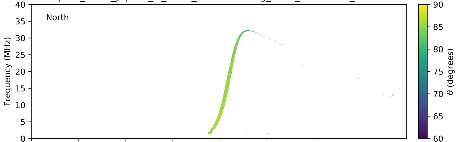
expres_earth_jupiter_io_isaac_lossc-wid1deg_1kev_20160501_v01.cdf
