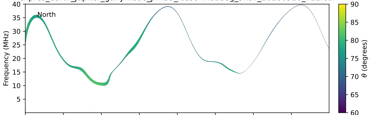
expres_earth_jupiter_ganymede_jrm33_lossc-wid1deg_3kev_20160526_v11.cdf
