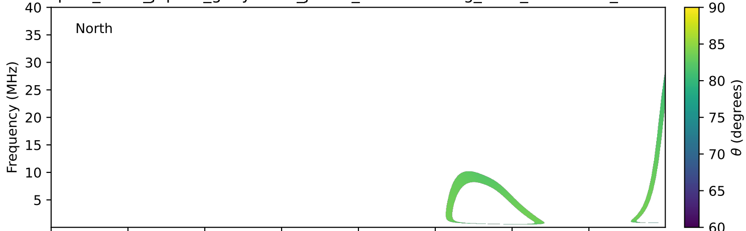
expres_earth_jupiter_ganymede_jrm33_lossc-wid1deg_3kev_20160525_v11.cdf
