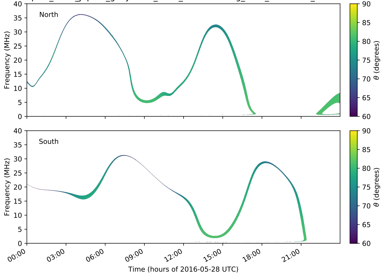
expres_earth_jupiter_ganymede_isaac_lossc-wid1deg_5kev_20160528_v01.cdf
