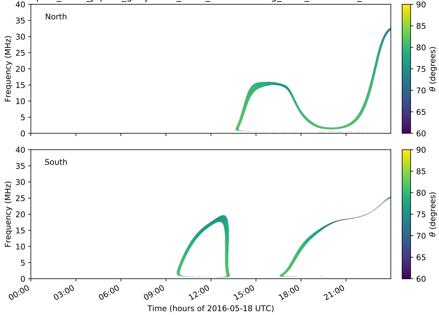
expres_earth_jupiter_ganymede_isaac_lossc-wid1deg_5kev_20160518_v01.cdf
