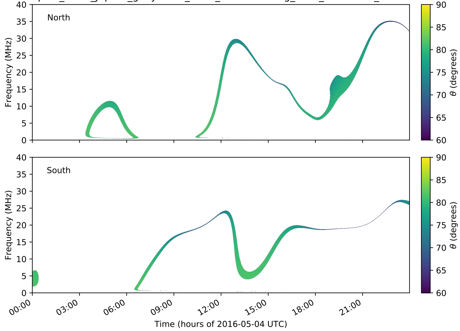
expres_earth_jupiter_ganymede_isaac_lossc-wid1deg_5kev_20160504_v01.cdf
