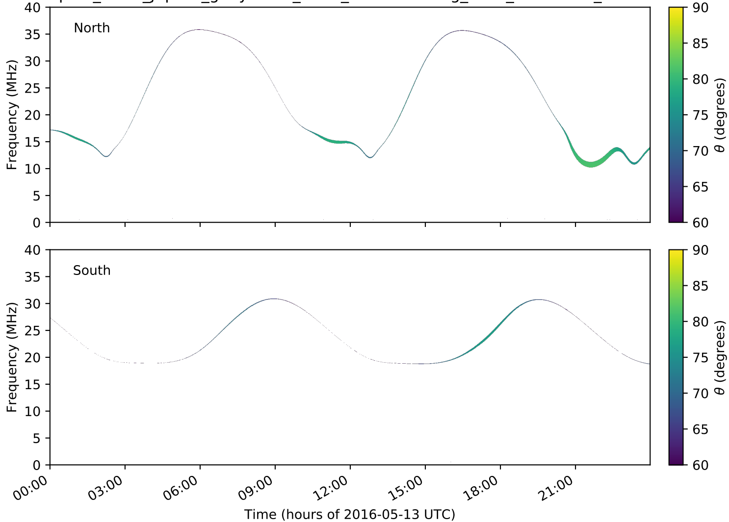
expres_earth_jupiter_ganymede_isaac_lossc-wid1deg_3kev_20160513_v01.cdf
