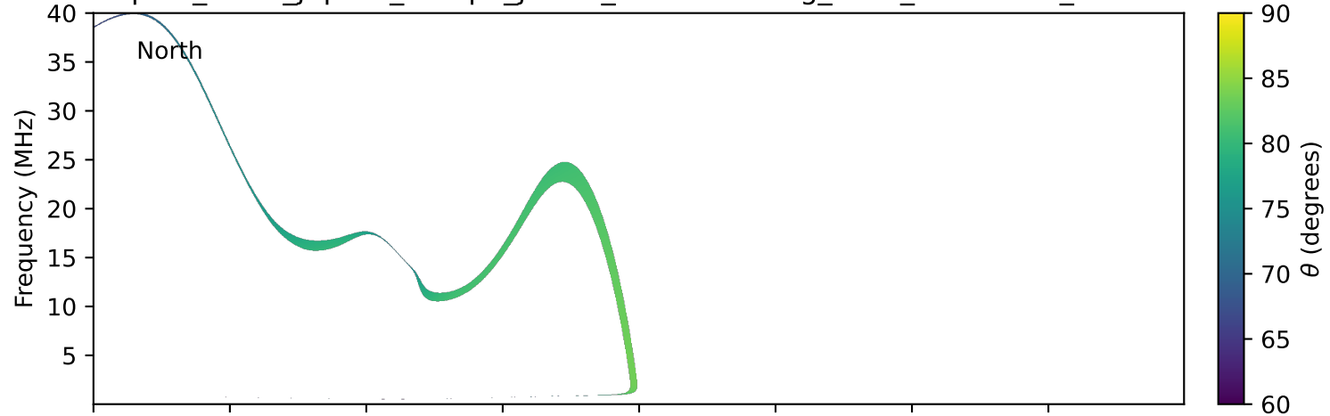
expres_earth_jupiter_europa_jrm33_lossc-wid1deg_3kev_20160529_v11.cdf
