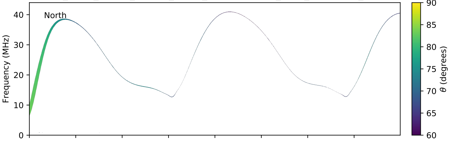
expres_earth_jupiter_europa_jrm09_lossc-wid1deg_3kev_20160528_v01.cdf
