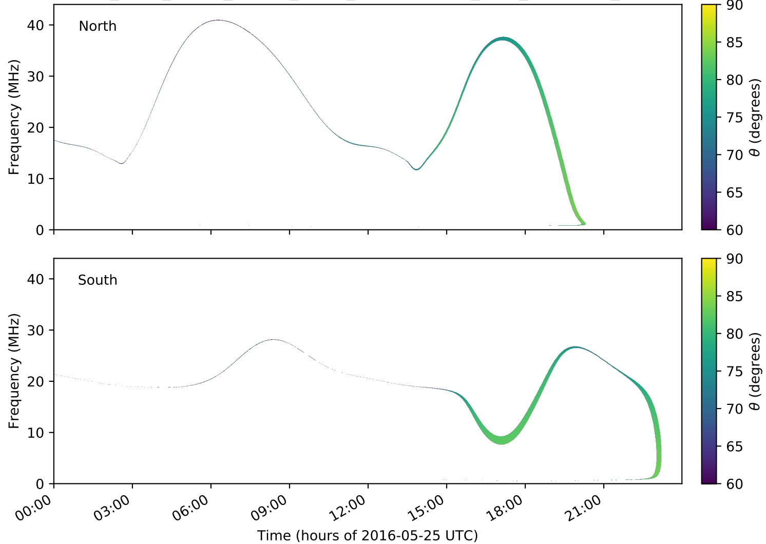
expres_earth_jupiter_europa_jrm09_lossc-wid1deg_3kev_20160525_v01.cdf
