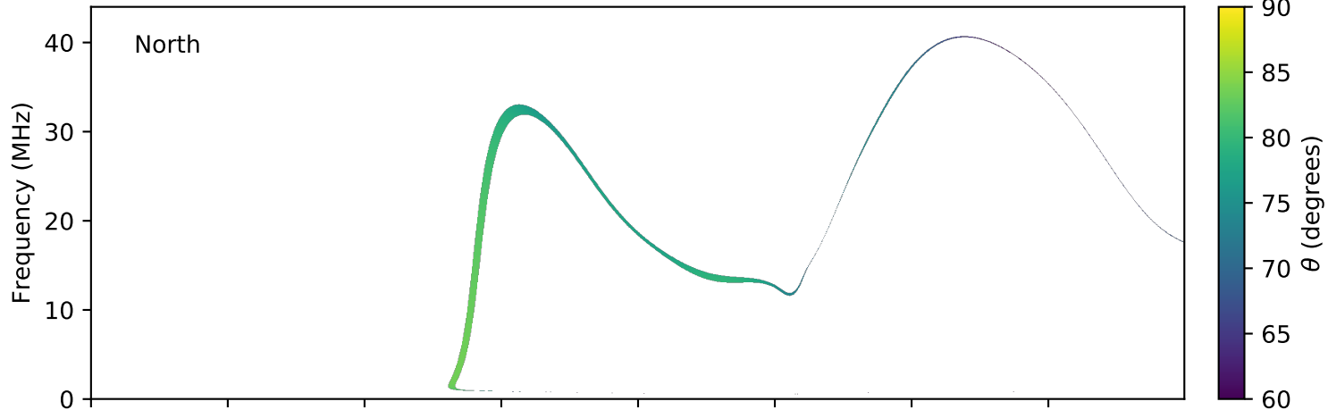
expres_earth_jupiter_europa_jrm09_lossc-wid1deg_3kev_20160524_v01.cdf
