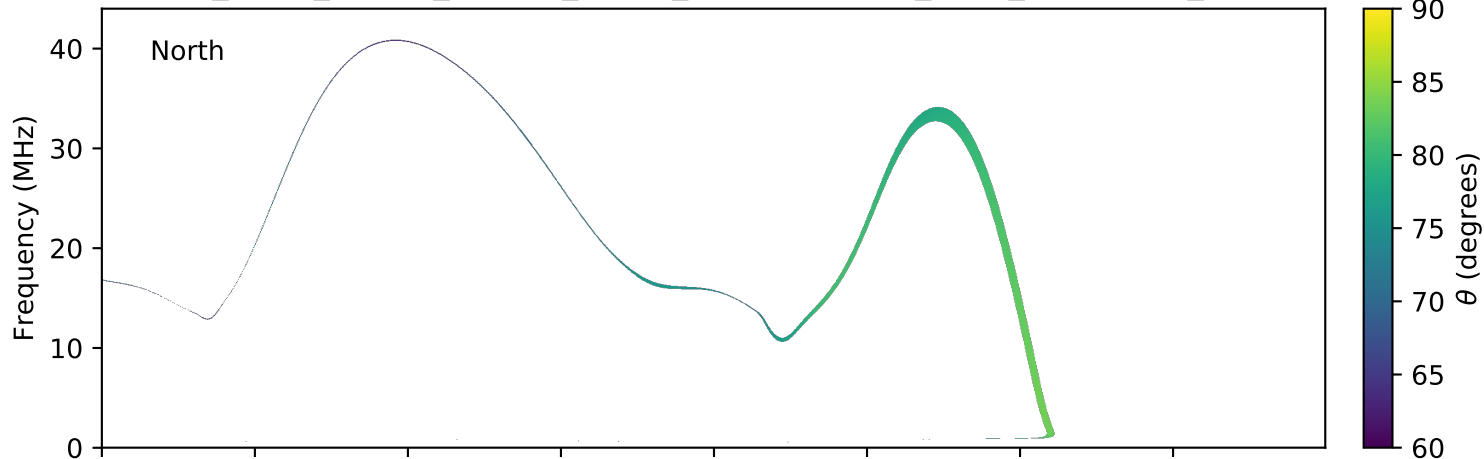
expres_earth_jupiter_europa_jrm09_lossc-wid1deg_3kev_20160518_v01.cdf
