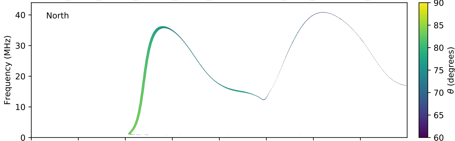
expres_earth_jupiter_europa_jrm09_lossc-wid1deg_3kev_20160517_v01.cdf
