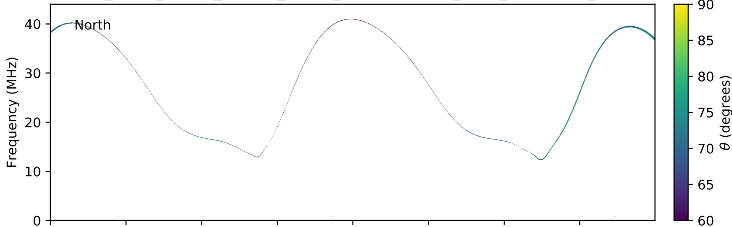
expres_earth_jupiter_europa_jrm09_lossc-wid1deg_3kev_20160514_v01.cdf
