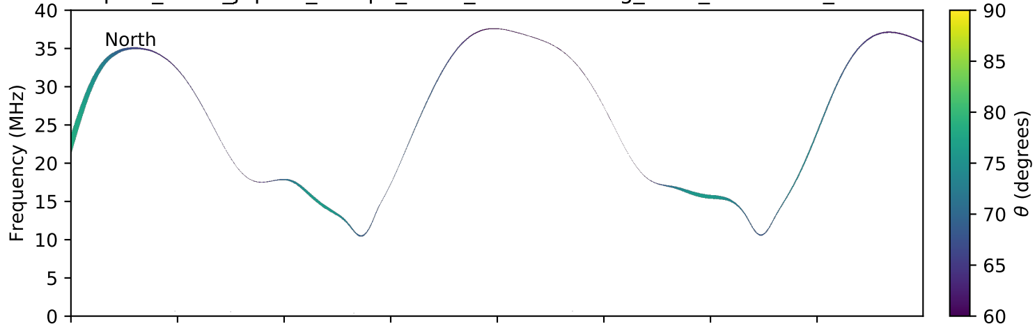
expres_earth_jupiter_europa_isaac_lossc-wid1deg_5kev_20160521_v01.cdf
