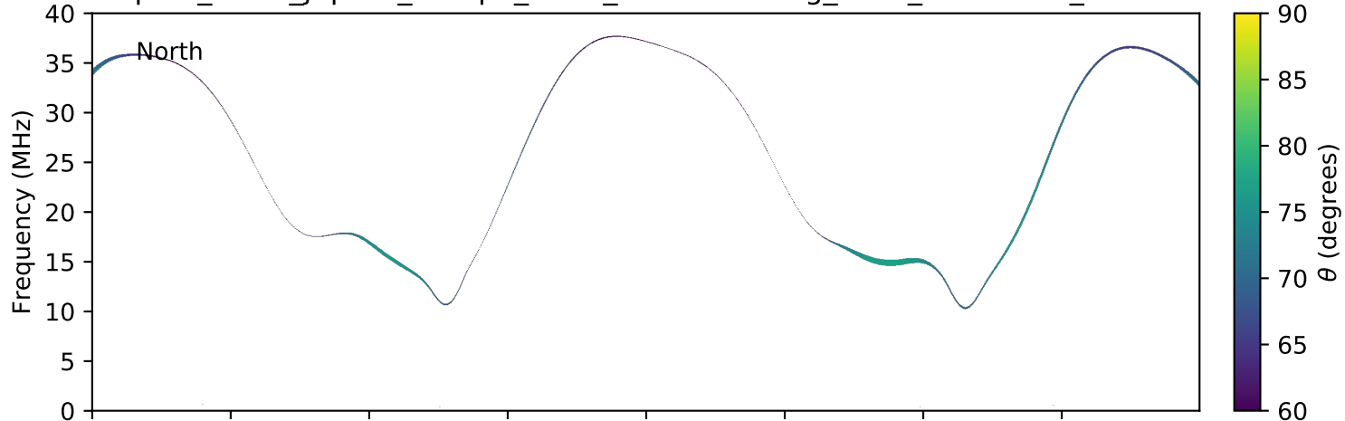
expres_earth_jupiter_europa_isaac_lossc-wid1deg_5kev_20160514_v01.cdf
